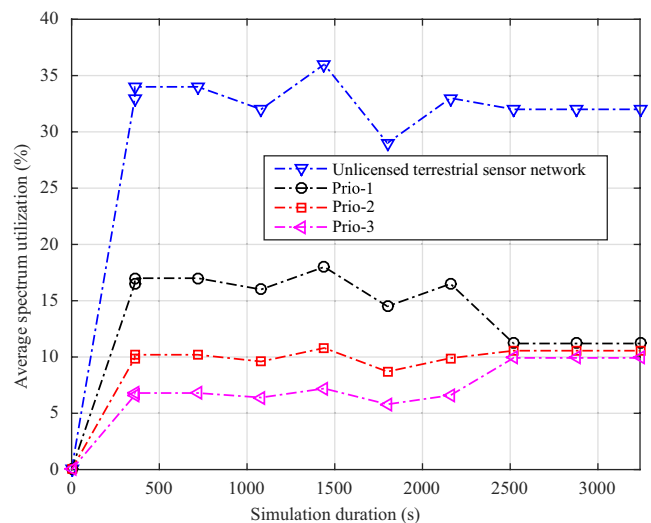
FIGURE 8 Spectrum utilization according to priority class
