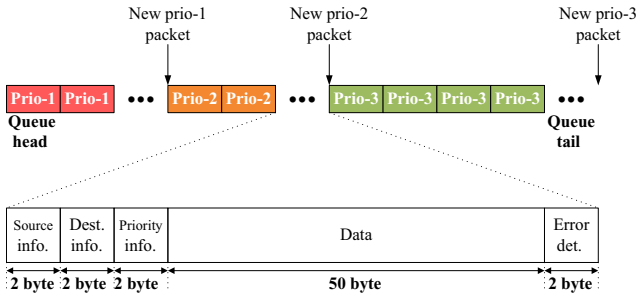
FIGURE 3 Unlicensed sensor node priority-based queue organization and packet structure
