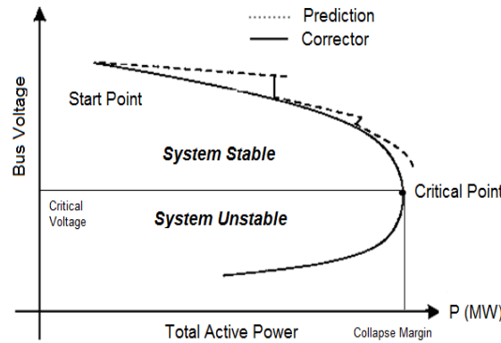
Figure 1. Predictive and corrective errors on the P-V curve
