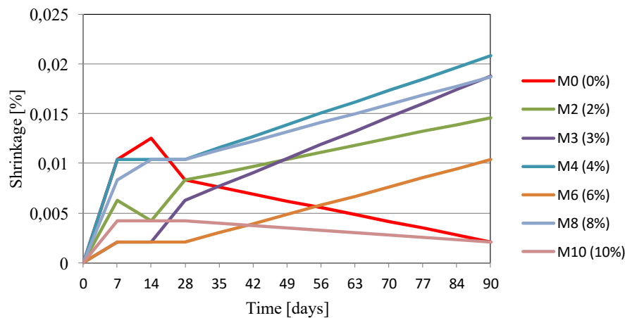
Figure 9. Shrinkage cement mortar with addition of basalt powder.
