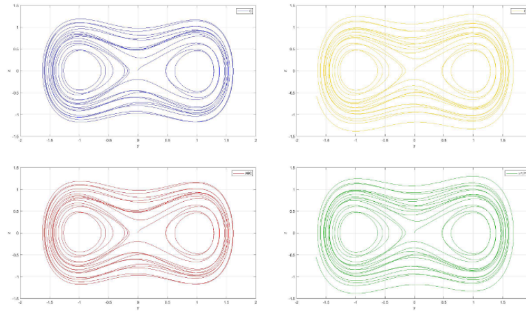
FIGURE 1. 2-D phase portraits for the numerical simulation for (21)
