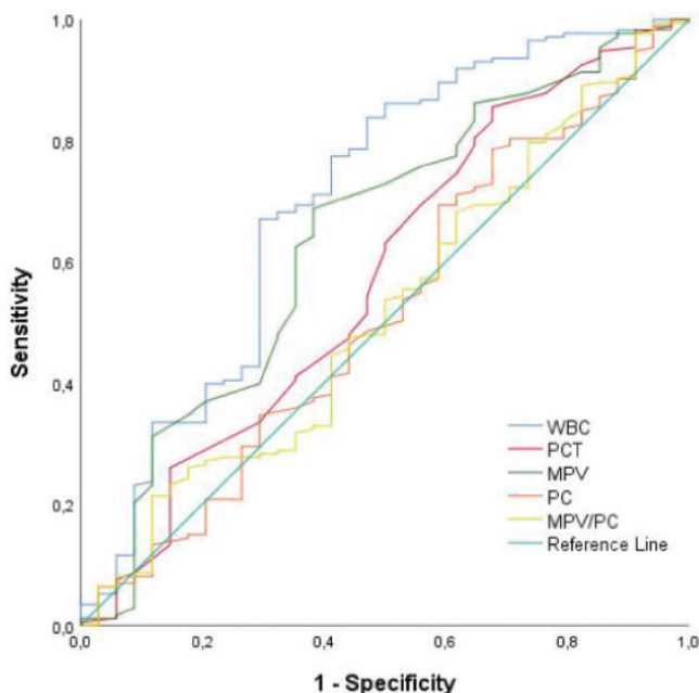
Figure 1. Receiver operating characteristic curve of parameters.
