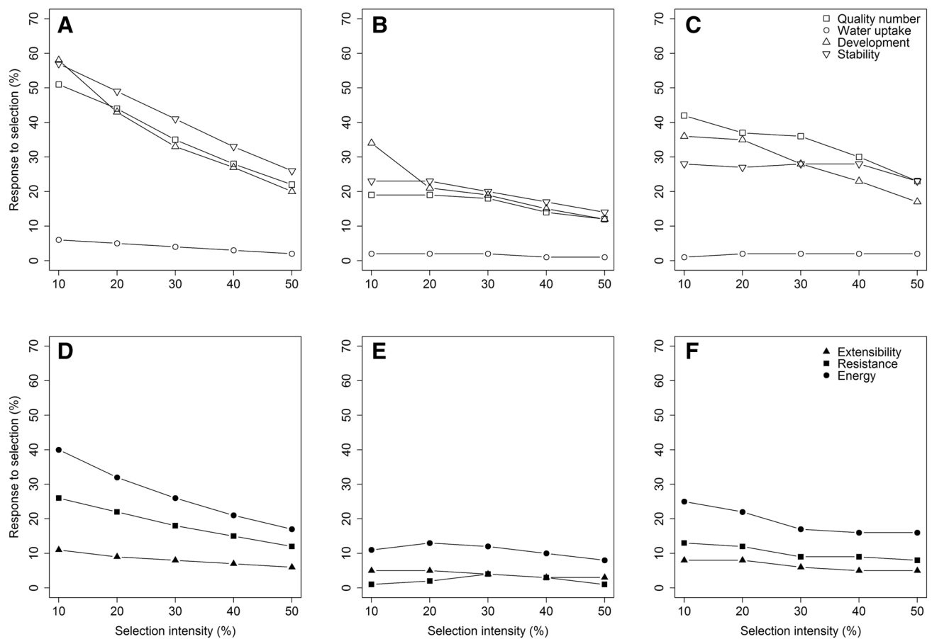
Fig. 6 Response to selection for the individual rheological traits using direct (a, d) and indirect phenotypic selection (b, e) as well as the model-based selection index approach that additionally included markers associated with the Glu-1 loci as fixed effects (c, f)
