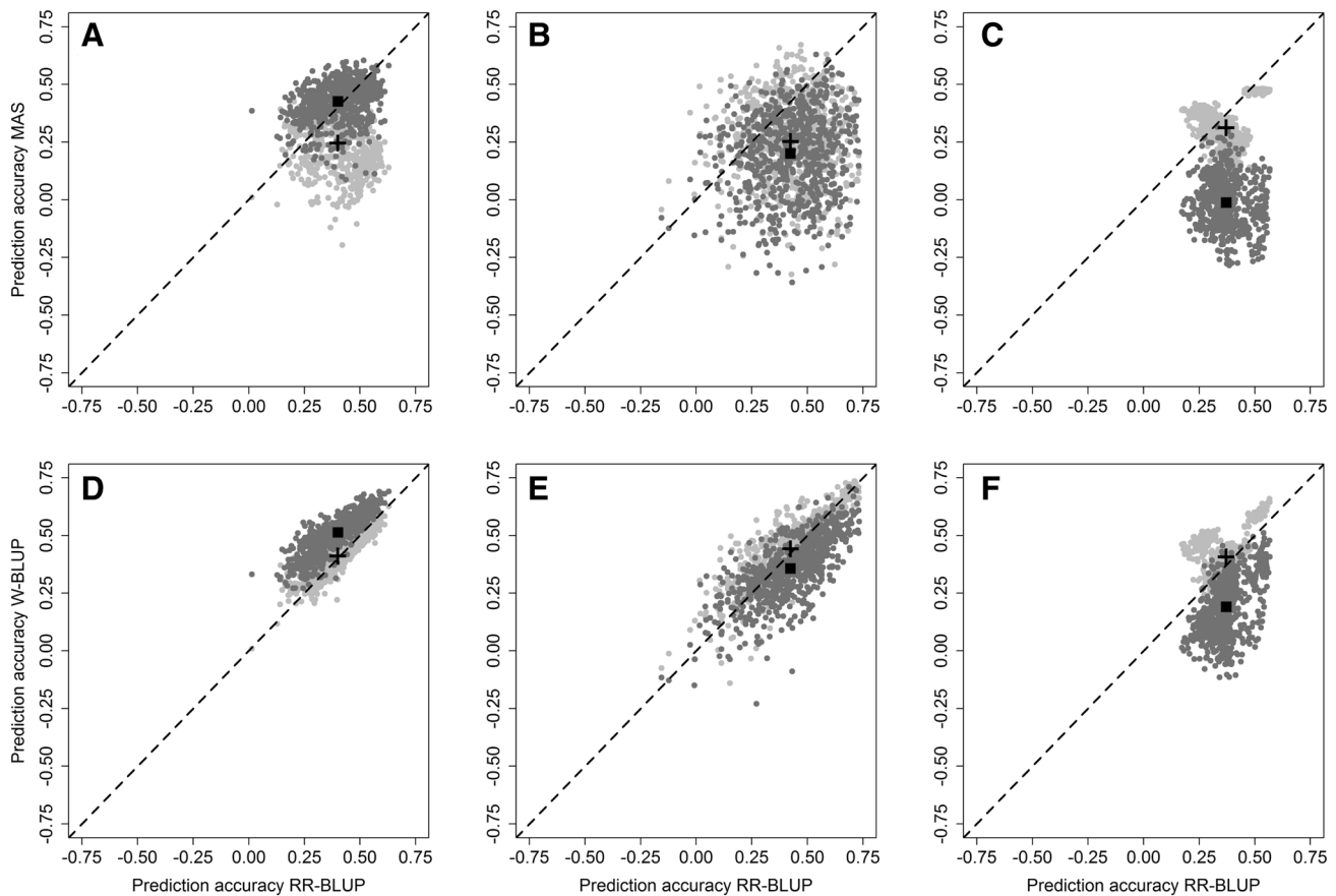
Fig. 2 Comparison between marker-assisted (top row) and genomic selection (bottom row) approaches employing markers linked with the Glu-1 loci (pale points) and de novo identified marker-trait associations (dark points), where each point represents a training by validation population by trait combination. Results are shown for the fourfold cross-validation within estimation set used for the GWAS
