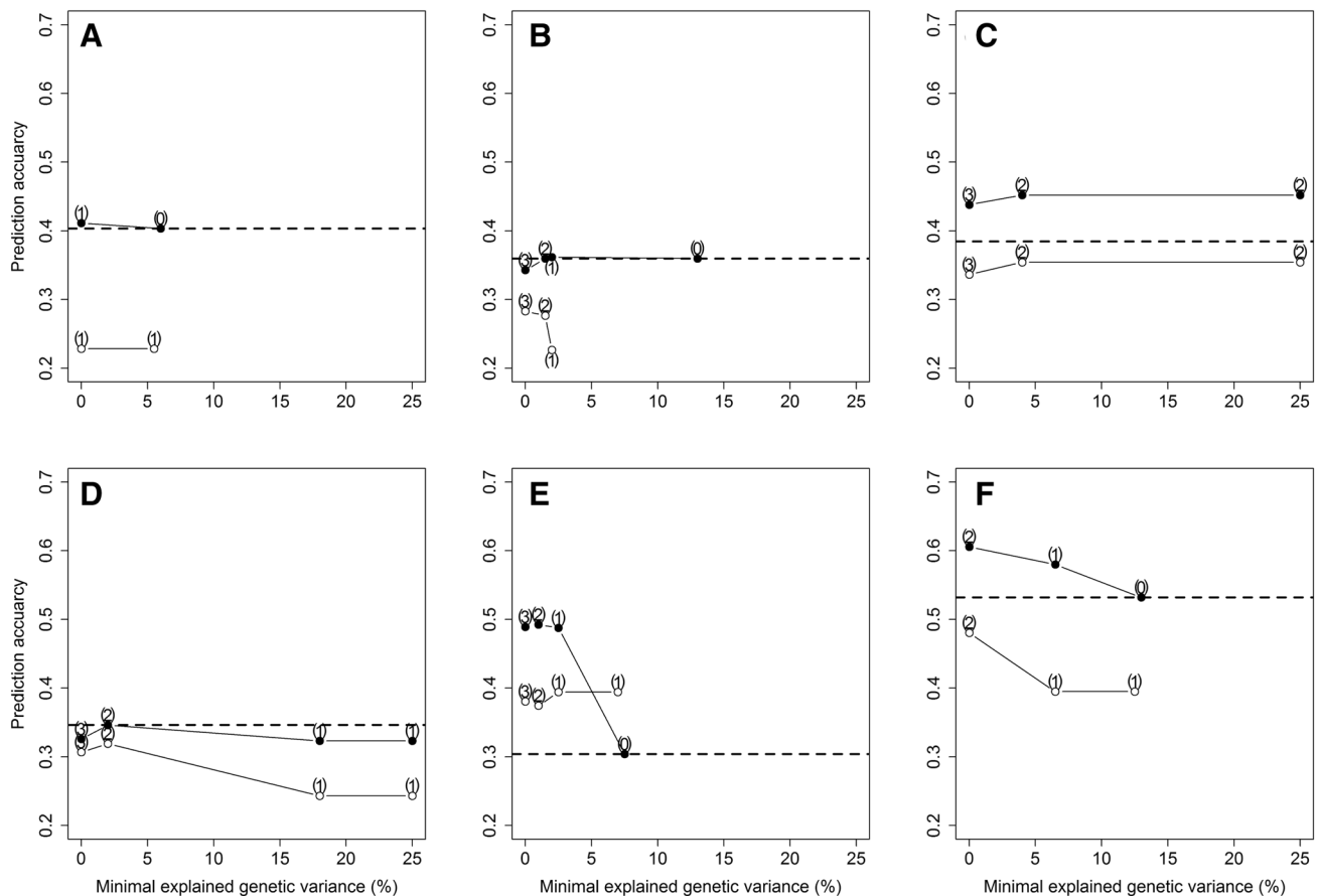
Fig. 3 The average prediction accuracy across all three independent validation populations 2014–2016 when training models for marker-assisted selection (open symbols) and integrating the Glu-1 loci as fixed effects into models for genomic selection (closed symbols). Different threshold values based on the explained genetic variance were applied for the water uptake (a), dough development (b), dough sta-
