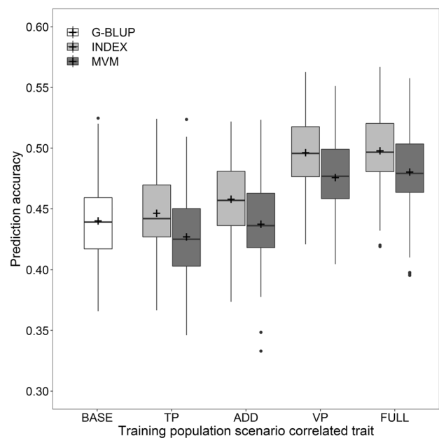
Fig. 4 Prediction accuracy for multi-trait genomic selection fitting a multi-trait mixed model (MVM) or employing a model-based selection index approach (INDEX), and the comparison with the corresponding single-trait prediction (G-BLUP). The baseline accuracy without modelling correlations between traits (BASE) was compared with multi-trait prediction scenarios where additional phenotypic data on the protein content was only available for the training population (TP), for both the training and validation population (VP), the training population as well as a large number of additional lines (ADD), and for all involved lines (FULL)
