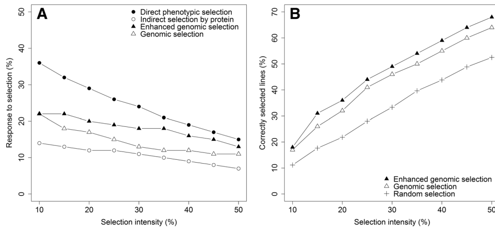
Fig. 5 Response to selection averaged across all analyzed dough rheological traits using direct and indirect phenotypic selection as well as the comparison with genomic selection and the advantage of using the model-based selection index approach that additionally included
