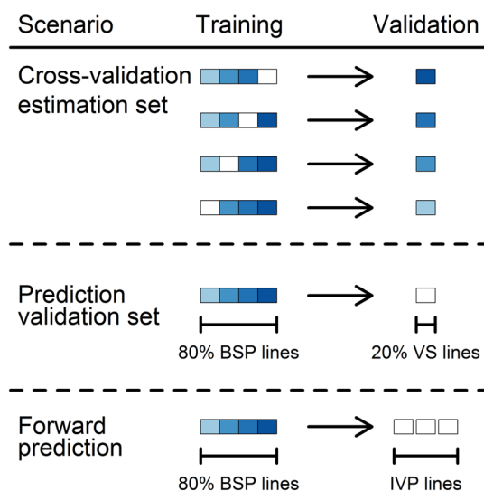
Fig. 1 Prediction scenarios used for the fourfold cross-validation within estimation set used for the GWAS in the basis population 2009–2013 (BSP), prediction of the validation set of the 20% of lines left-out for the GWAS (VS), and the forward prediction of the three independent validation populations 2014–2016 (IVP)
