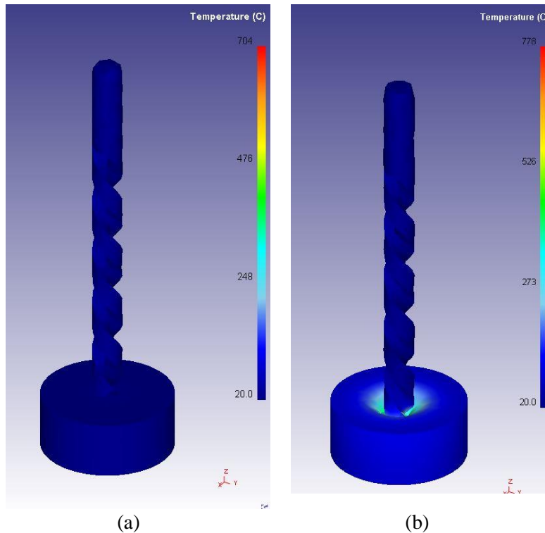
Figure 5. Temperature estimates of the drilling simulation a) \epsilon=118^\circ , b) \epsilon=135^\circ
