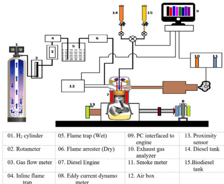
FIGURE 1 Engine setup schematic arrangement in the study
