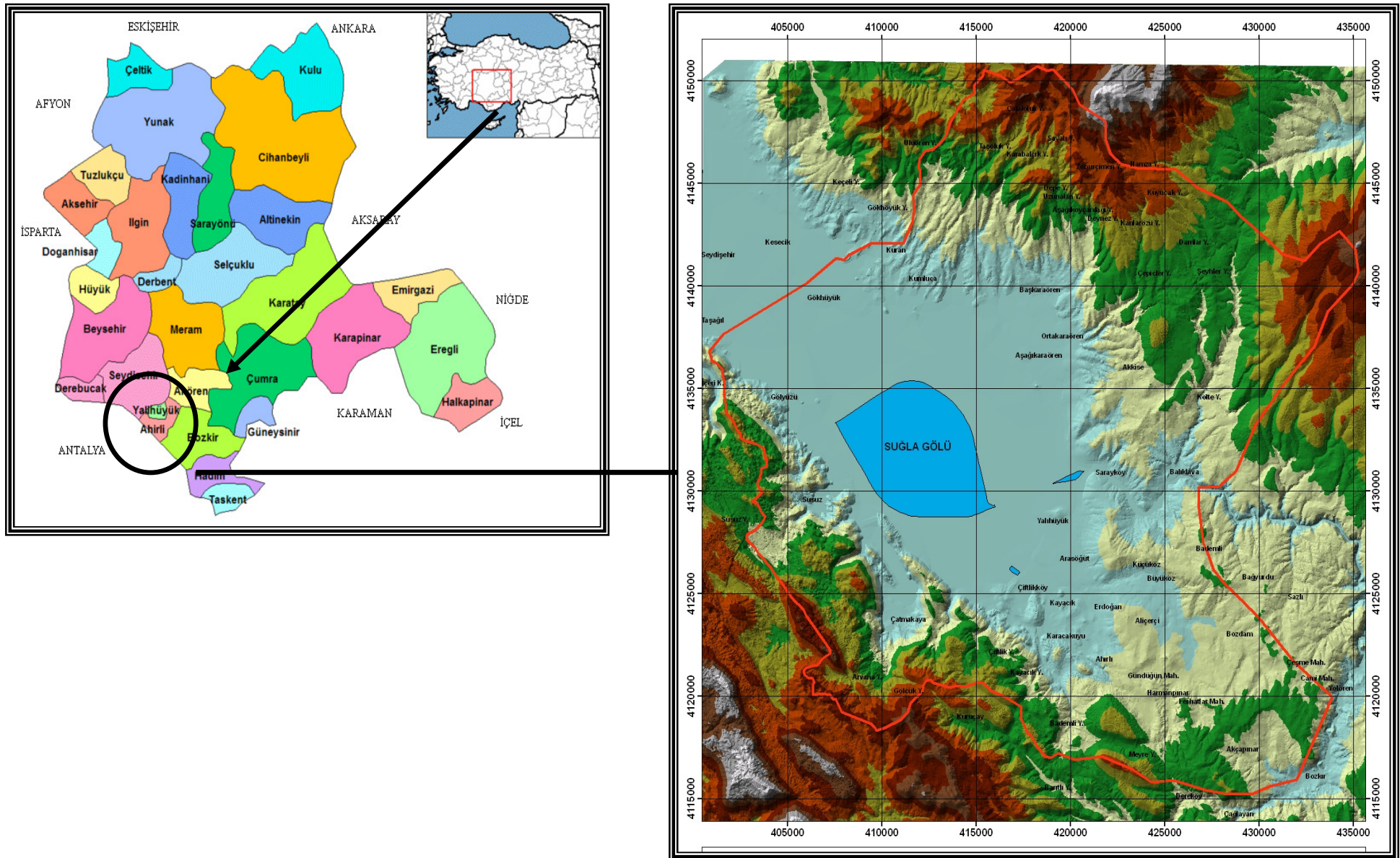
Figure 1. Study area
