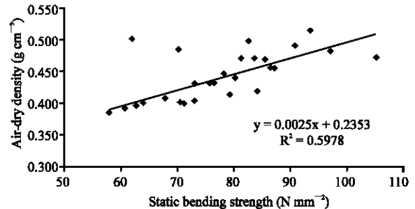
Fig. 2: The relationship between static bending strength and air-dry density
