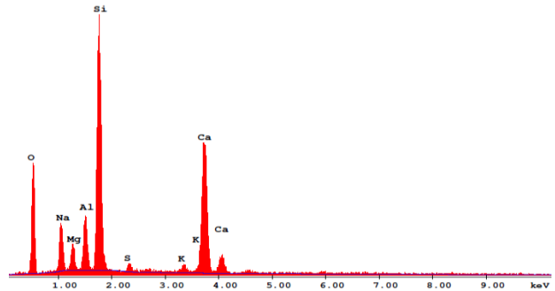
Figure 7. EDS analysis of Mix2
