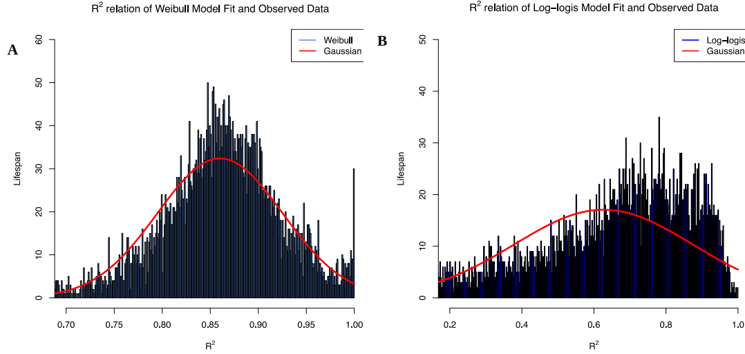
Figure 3. (A) Histogram of R^2 \sim [70\%, 100\%] between WE model and empirical lifespan of each RLS of all the genetic backgrounds in the data set. (B) Histogram of R^2 \sim [20\%, 100\%] between Log-logis and lifespan of each RLS of all the genetic backgrounds in the same data set. This relation between the WE model and empirical data shows a tendency to a Gaussian curve which shows a better fit and model for the yeast lifespan samples.
