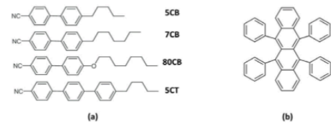
Figure 1. The molecular formula of the (a) E7 NLC and (b) Rubrene fluorescent dye.
