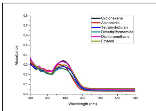
Figure 7. Absorption spectrum of 3c
