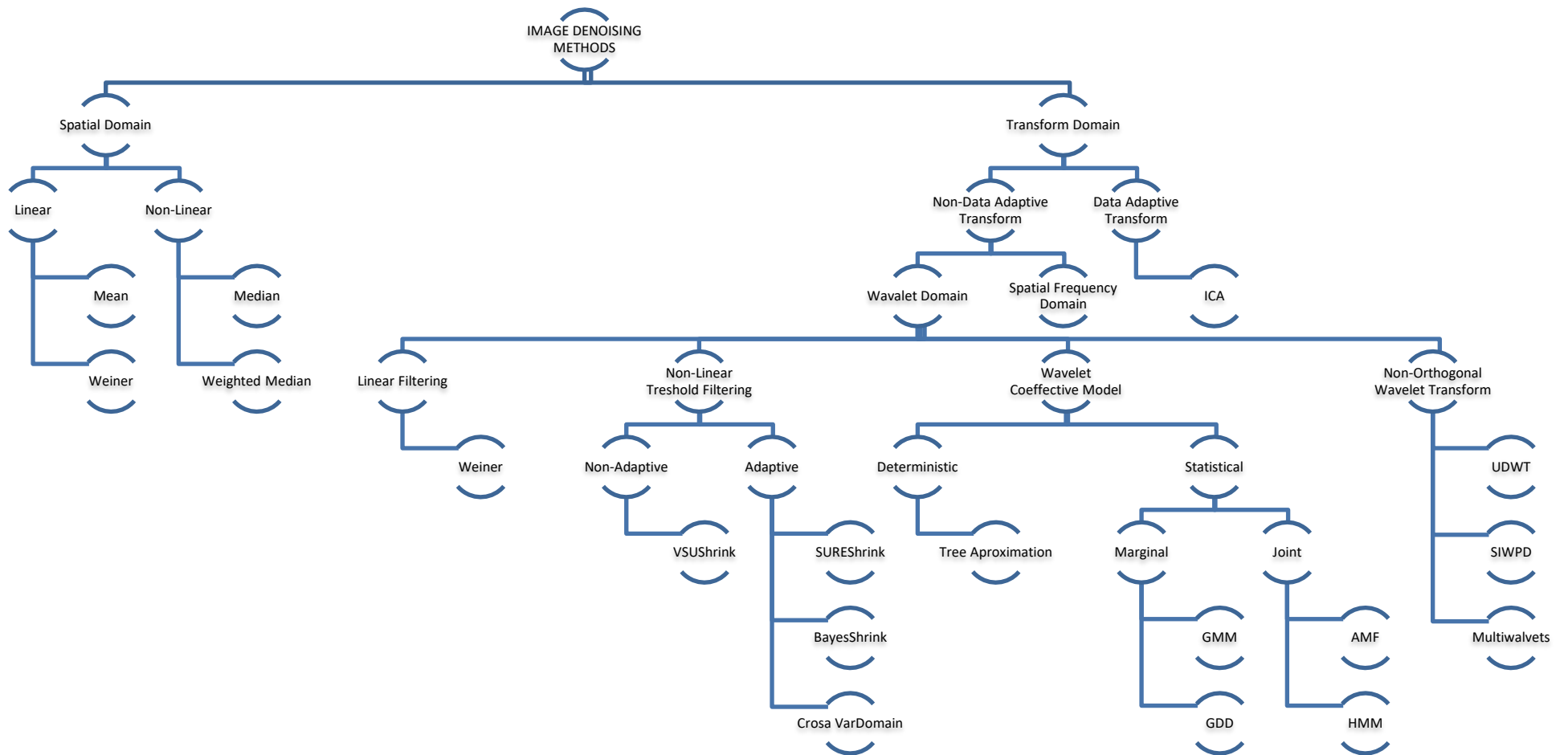
Figure 1. Image denosing methods
