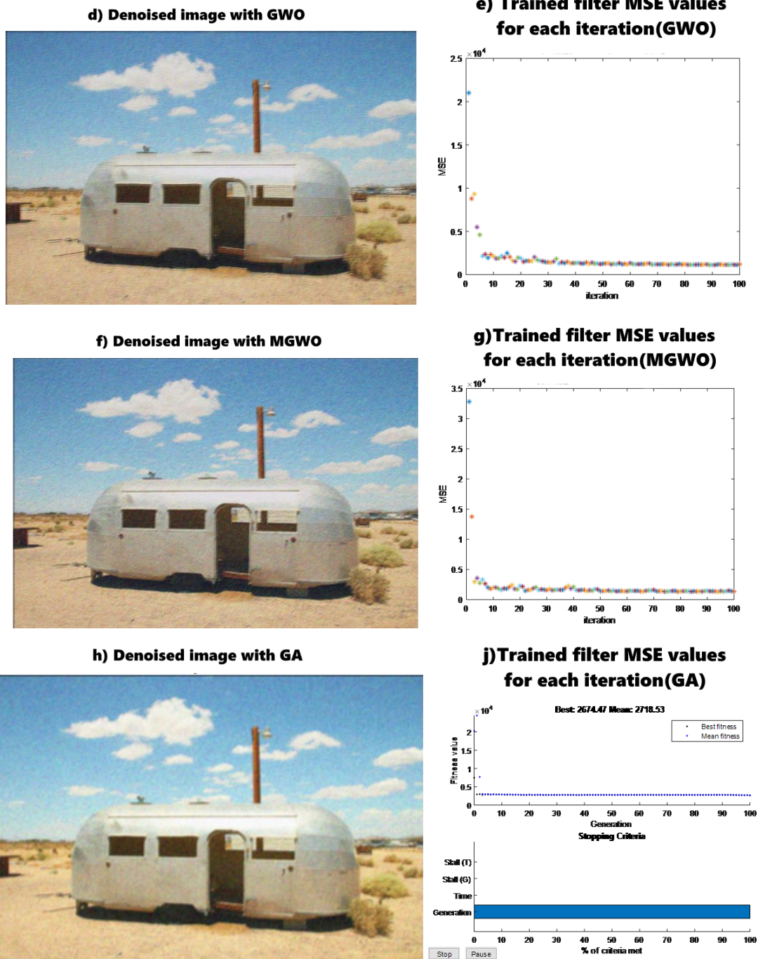
Figure 5. a) Original image(Trailer), b) Gaussian Noisy image \mu=0.1 , \sigma=0.02 , c) Denoised image with Weiner, d) Denoised image with GWO, e) Trained filter MSE values for each iteration(GWO), f) Denoised image with MGWO, g) Trained filter MSE values for each iteration(MGWO), h) Denoised image with GA, j) Trained filter MSE values for each iteration(GA)
