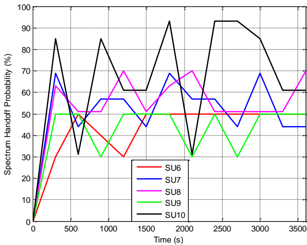
Figure 5. Spectrum handoff probabilities according to the medium usage intensity of primary users.
