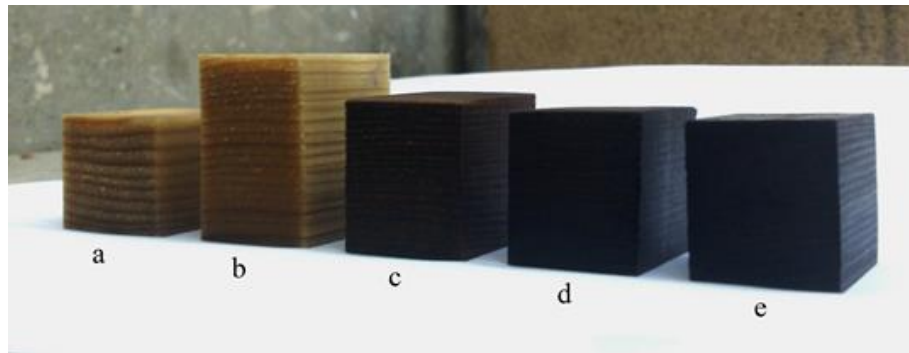
Fig. 2. The appearance of samples after soaking in water (a: control; b: densified; c: densified + treated at 190 °C; d: densified + treated at 200 °C; e: densified + treated at 210 °C)
