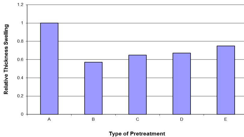
Fig. 4. Effects of different pretreatments on the thickness swelling of wheat straw particleboards
