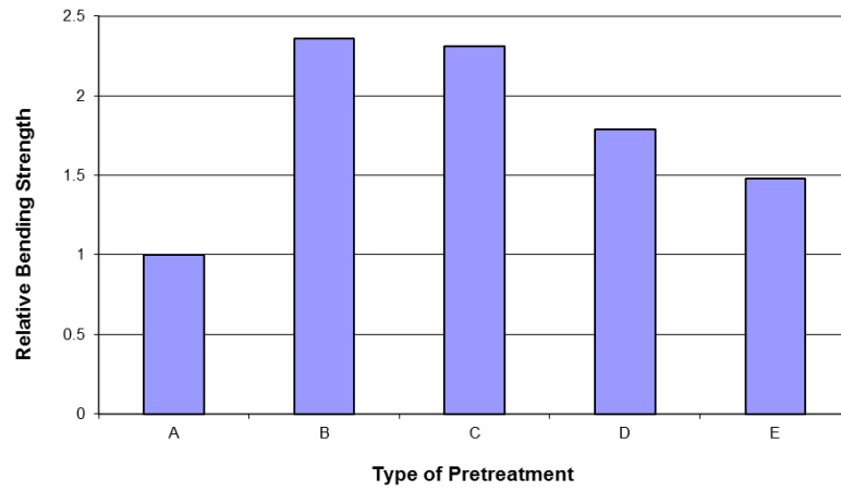
Fig. 1. Effects of different pretreatments on the bending strength of wheat straw particleboards
