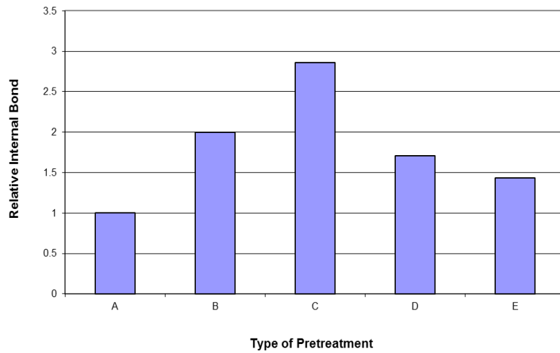
Fig. 2. Effects of different pretreatments on the internal bonds in wheat straw particleboards
