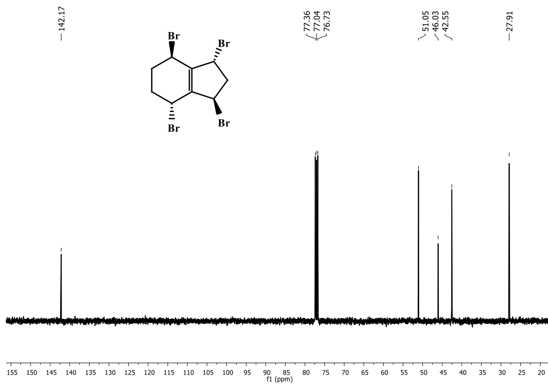
Figure S2. ^{13}\text{C} -NMR Spectrum of compound 12 .
