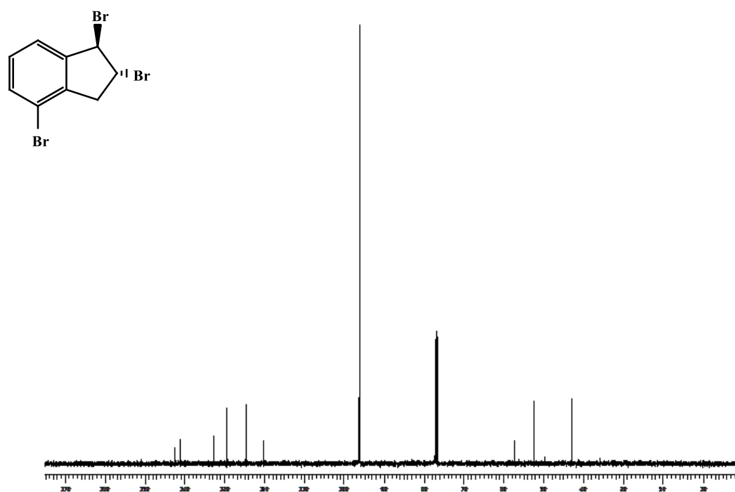
Figure S22. ^{13}\text{C} -NMR Spectrum of compound 16.
