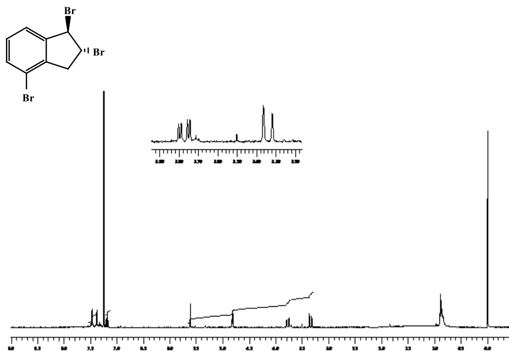
Figure S21. ^1\text{H} -NMR Spectrum of compound 16.
