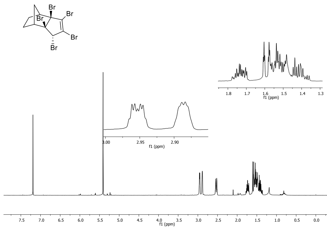
Figure S27. 1 H-NMR Spectrum of compound 23.
