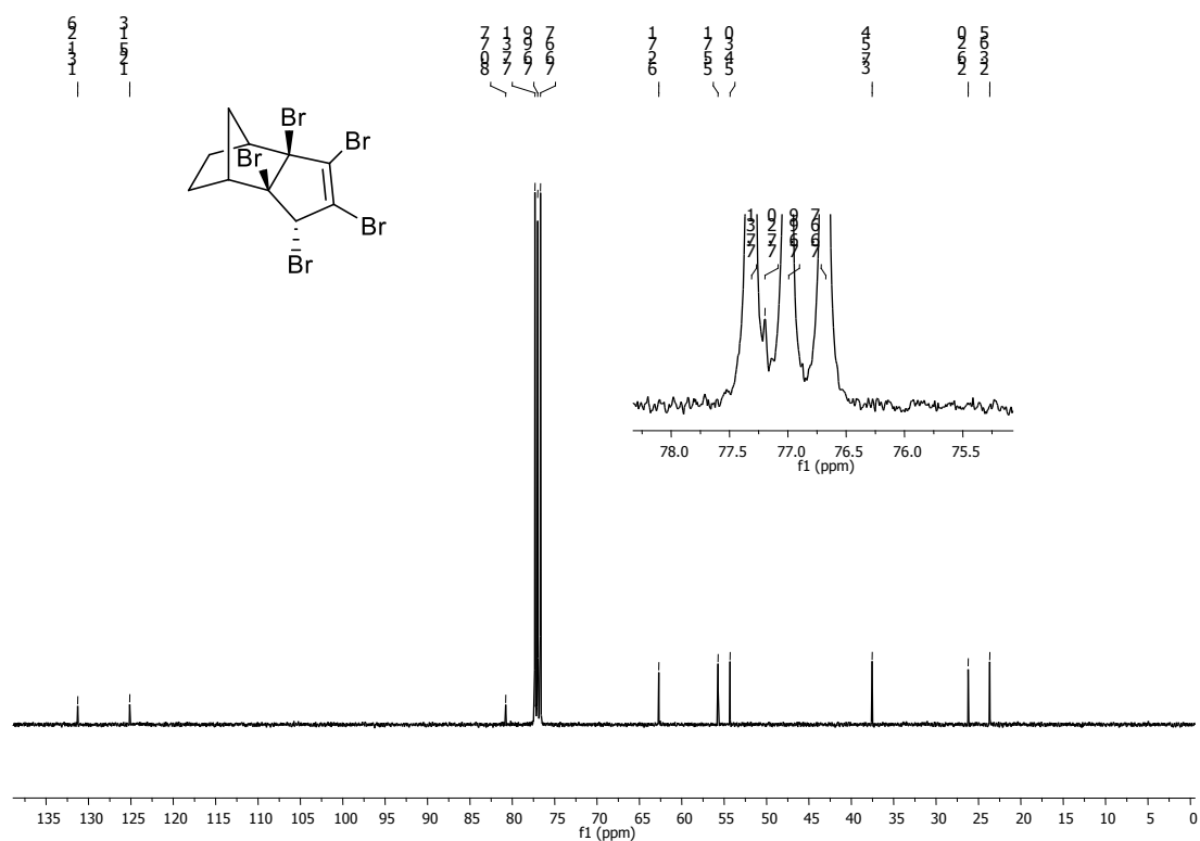
Figure S28. 13 C-NMR Spectrum of compound 23.
