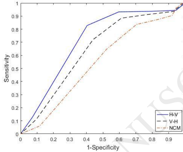
Fig. 5. Segmentation evaluation using the ROC curve
