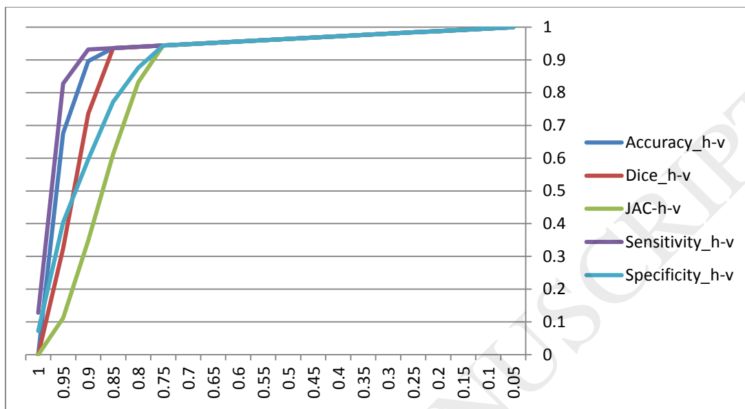
Fig. 8. The CP of the different metrics with using the HBCENCM method using with h-v procedure
