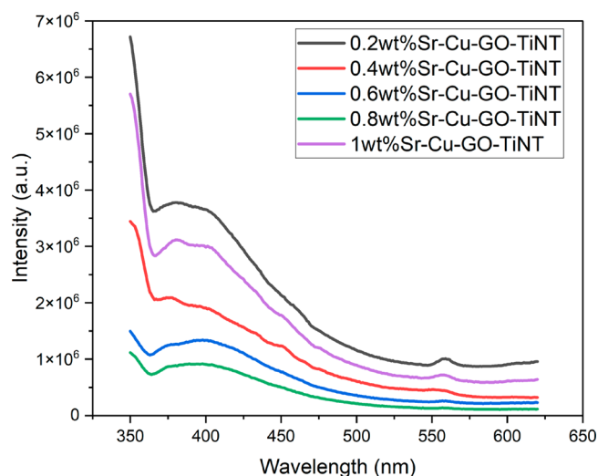
Figure 8. Photoluminescence spectra of the x\text{wt}\%\text{Sr-Cu-GO-TiNT} materials with x varying between 0.2 and 1.0 wt % Sr.
