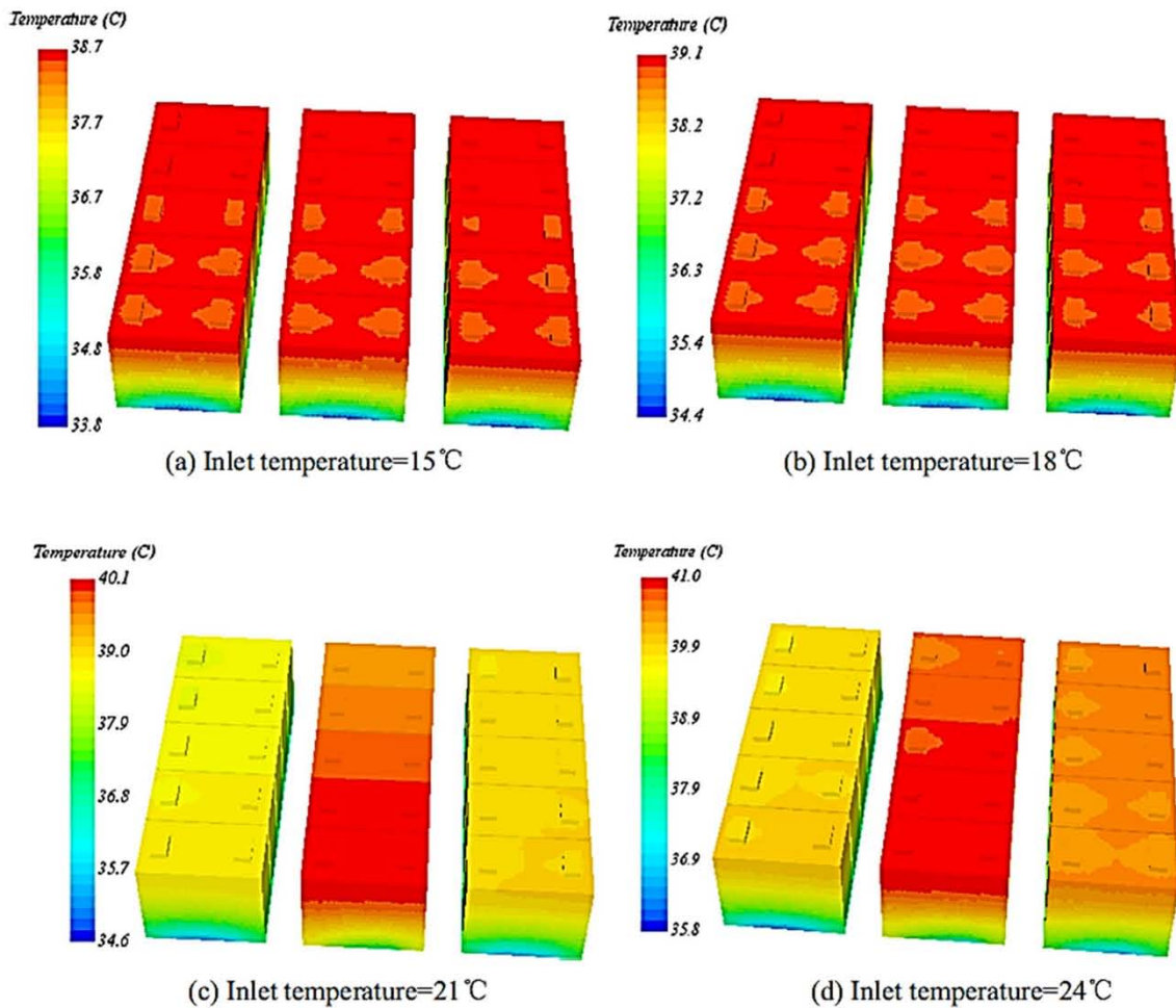
Fig. 78 Temperature contours in battery module at constant cooling plate width and varying inlet temperature a inlet temperature= 15 °C, b inlet temperature= 18 °C, c inlet temperature=21 °C, d inlet temperature= 24 °C [145]
