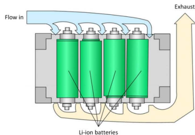
Fig. 8 Forced air cooling system [58]
