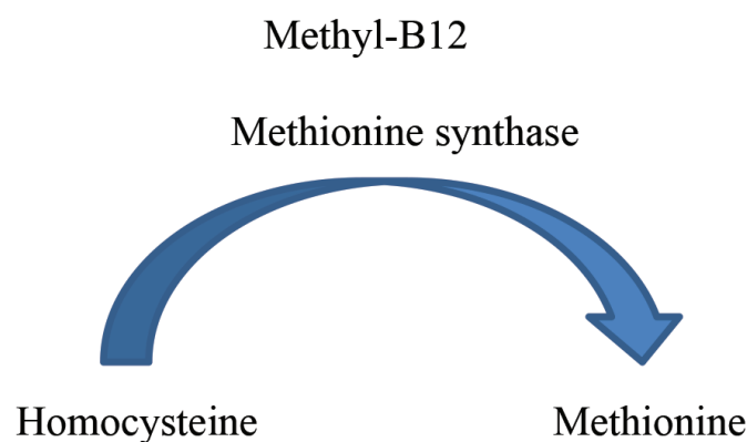
Figure 1. Homocysteine metabolism
