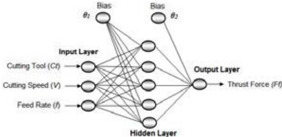
Fig. 1. ANNs architecture with a single hidden layer
