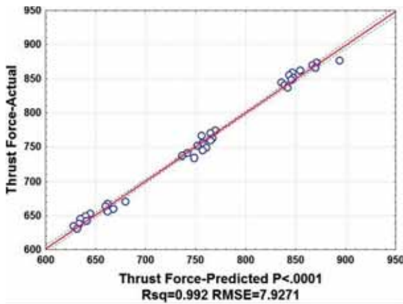
Fig. 3. Comparison of experimental and residual thrust forces with thrust forces predicted by regression analysis
