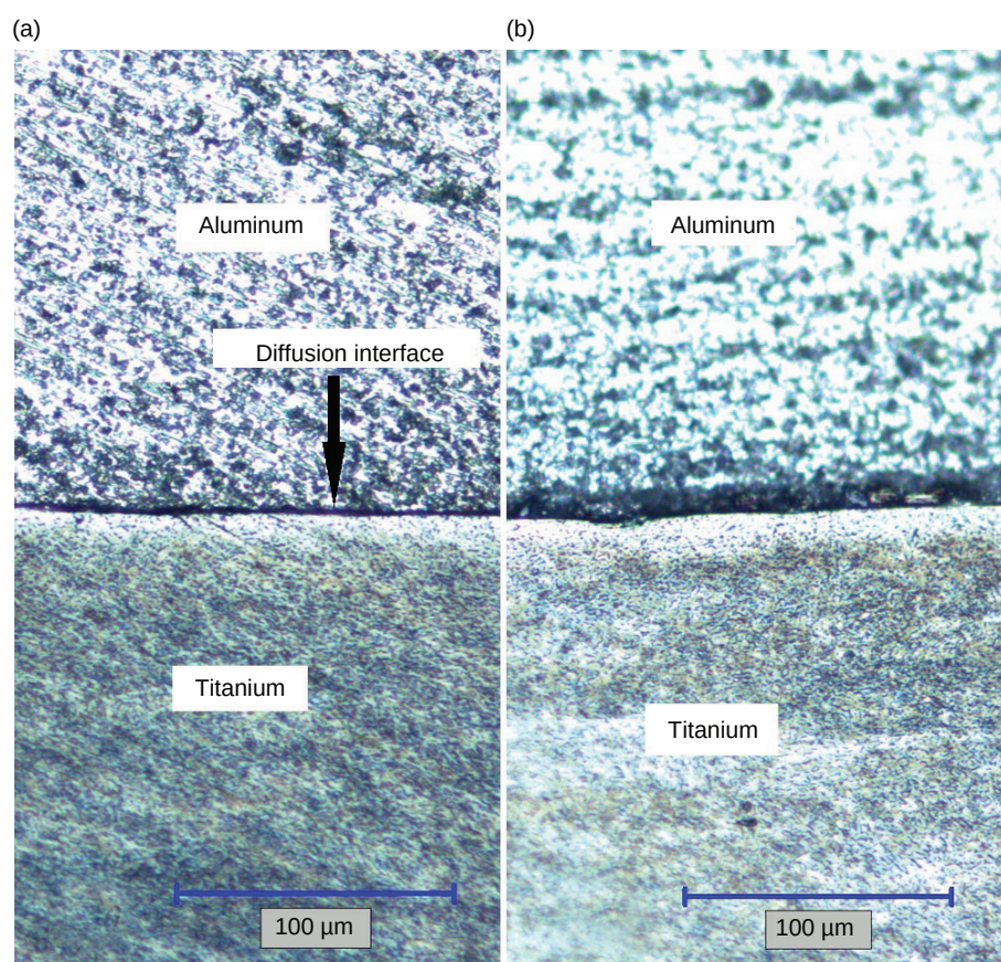
FIGURE 3. Optical micrograph of the sample bonded at 560 °C for 60 min at the atmosphere of: (a) argon gas and (b) non-argon.
