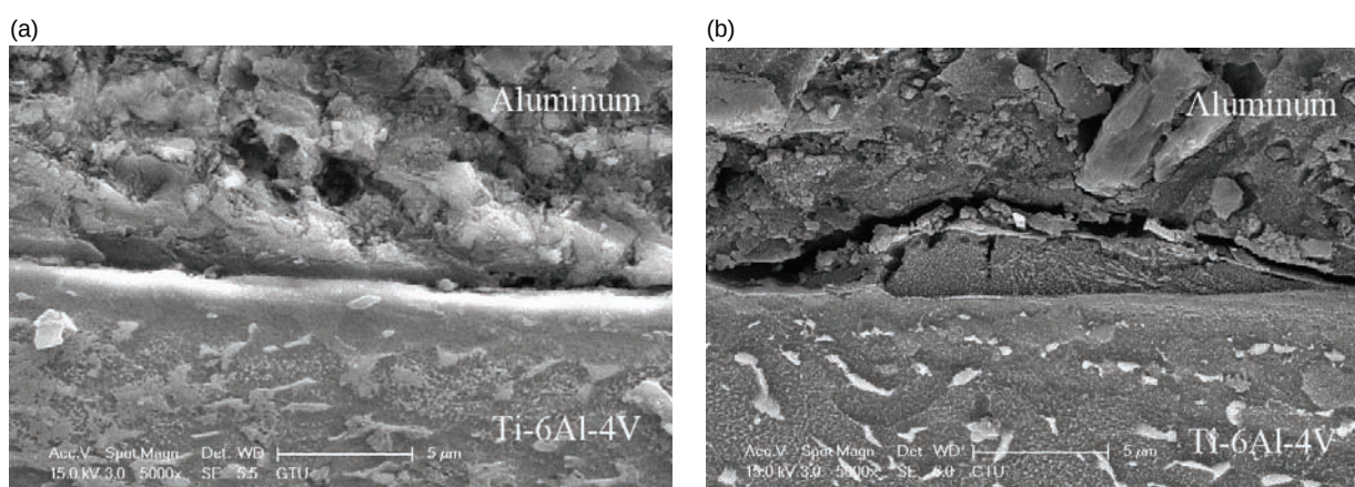
FIGURE 10. SEM micrograph of the sample bonded at 640 °C for 60 min at the atmosphere of: (a) argon gas and (b) non-argon.
