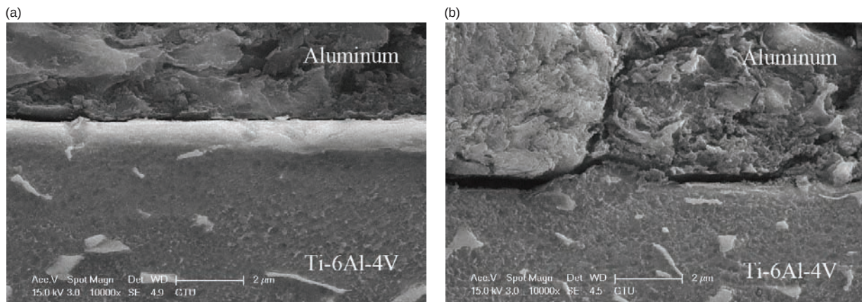
FIGURE 7. SEM micrograph of the sample bonded at 560 °C for 60 min at the atmosphere of: (a) argon gas and (b) non-argon.
