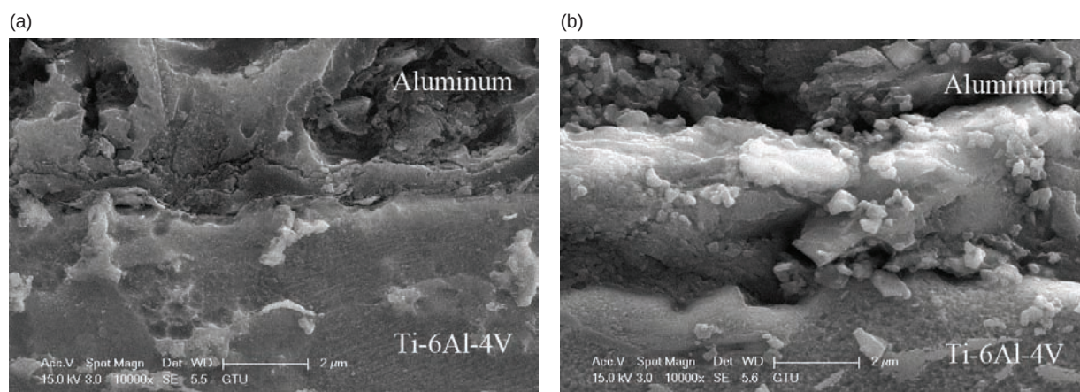
FIGURE 8. SEM micrograph of the sample bonded at 600 °C for 30 min at the atmosphere of (a) argon gas and (b) non-argon.
