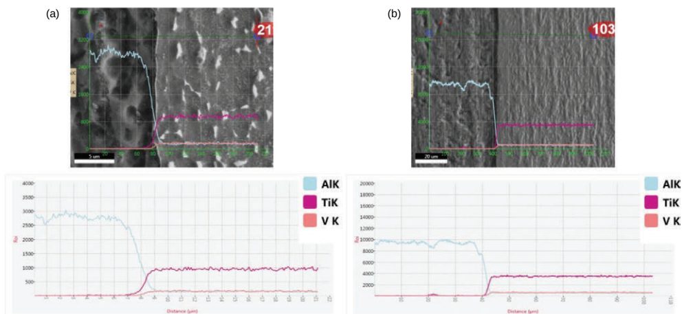
FIGURE 12. EDS line element analysis of the samples bonded at 600 °C for 60 min at the atmosphere of: (a) argon gas and (b) non-argon.
