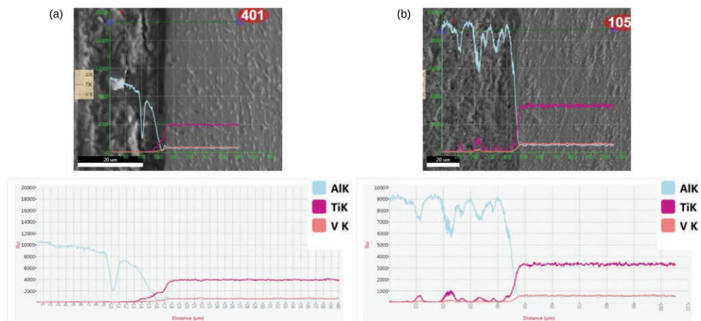
FIGURE 14. EDS line element analysis of the samples bonded at 640 °C for 45 min at the atmosphere of: (a) argon gas and (b) non-argon.
