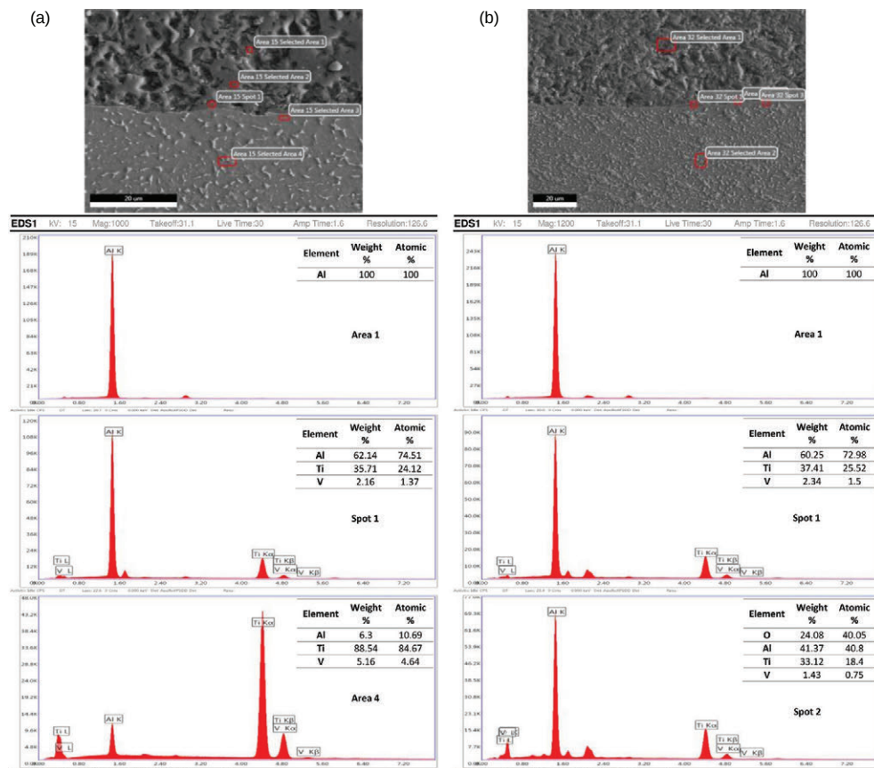
FIGURE 13. EDS elemental composition of selected areas of the samples bonded at 640 °C for 45 min at the atmosphere of: (a) argon gas and (b) non-argon.
