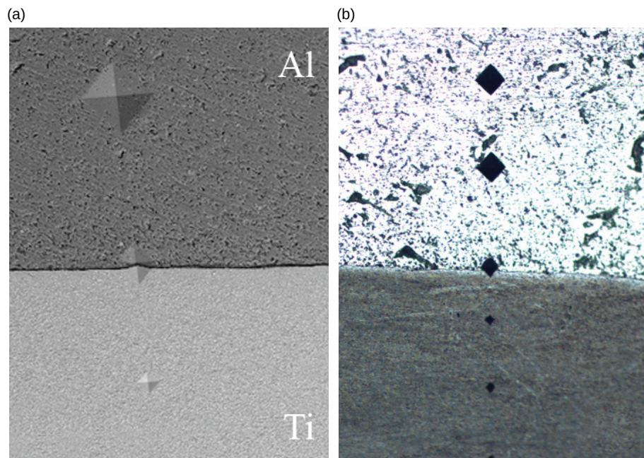
FIGURE 15. Microhardness measurement marks with; a) SEM and b) optical micrographs.
