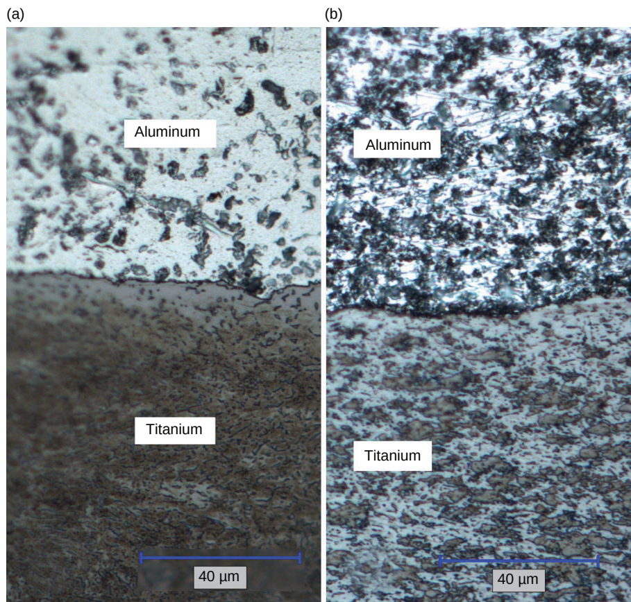
FIGURE 6. Optical micrograph of the sample bonded at 640 °C for 30 min at the atmosphere of: (a) argon gas and (b) non-argon.
