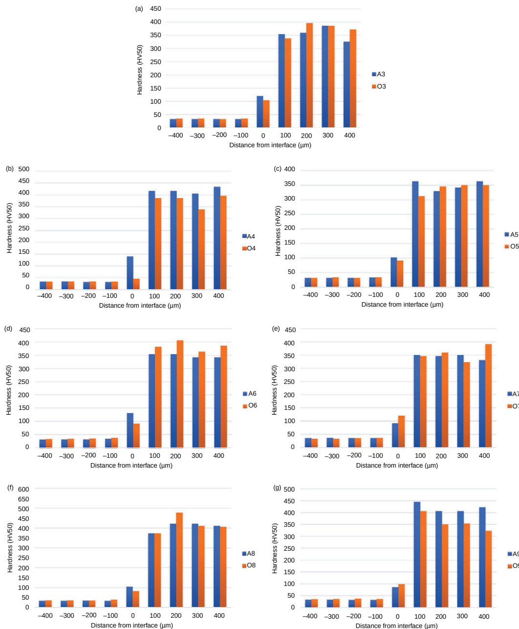
FIGURE 16. Hardness profiles of all bonded samples.
