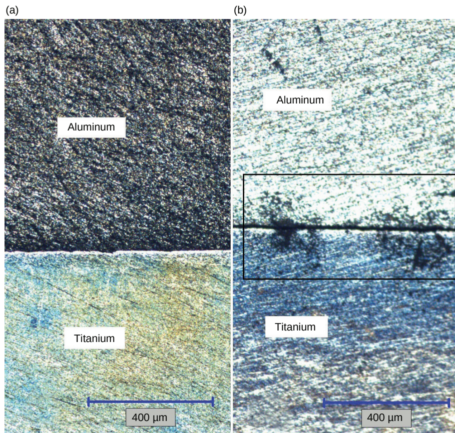
FIGURE 4. Optical micrograph of the sample bonded at 600 °C for 30 min at the atmosphere of: (a) argon gas and (b) non-argon.
