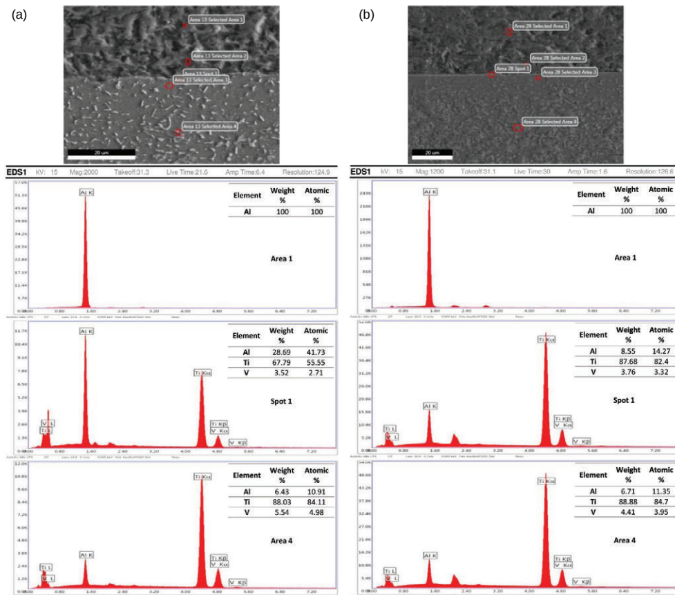
FIGURE 11. EDS elemental composition of selected areas of the samples bonded at 600 °C for 60 min at the atmosphere of: (a) argon gas and (b) non-argon.
