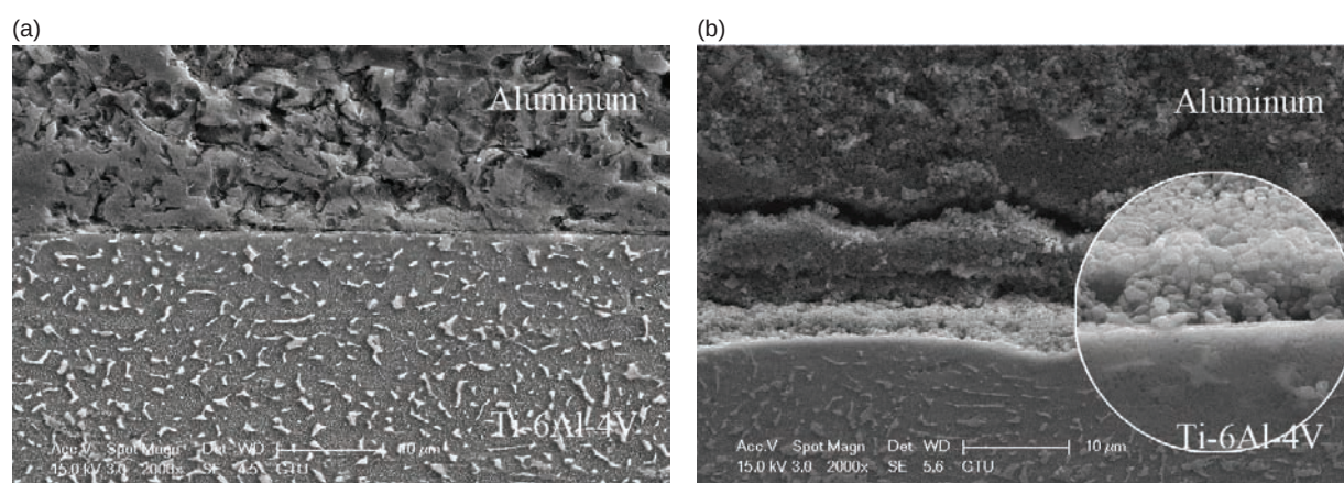
FIGURE 9. SEM micrograph of the sample bonded at 600 °C for 45 min at the atmosphere of: (a) argon gas and (b) non-argon.
