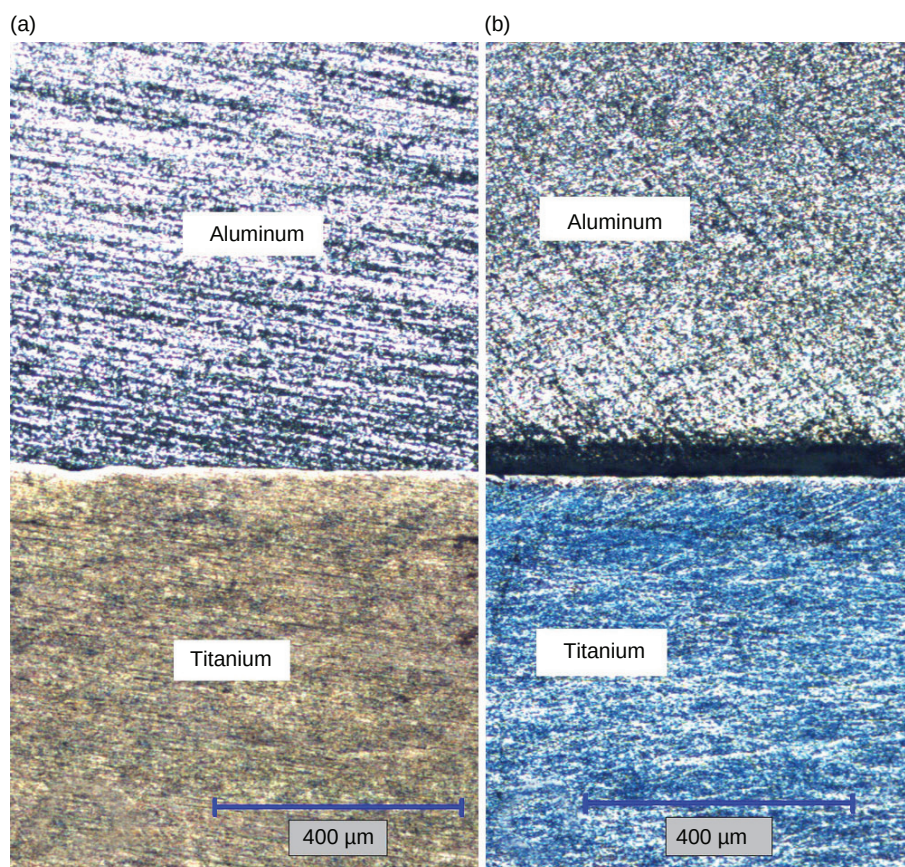
FIGURE 5. Optical micrograph of the sample bonded at 600 °C for 45 min at the atmosphere of: (a) argon gas and (b) non-argon.
