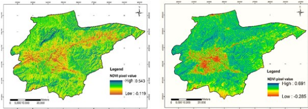
Figure 2. NDVI satellite image of 1990 was obtained from Landsat 5 satellite image (left) and the NDVI satellite image of 2018 was obtained from Landsat 8 satellite image (right)
